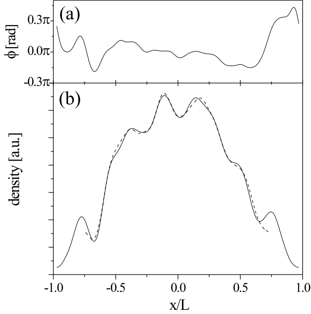
Figure 6.2.2: (a) A typical initial phase distribution calculated for \omega_x = 2\pi \times 14 \text{ Hz} , \omega_\rho = 2\pi \times 508 \text{ Hz} , N_0 = 2 \times 10^5 , and T = 0.5 T_c . (b) Corresponding density profile after 25 ms time-of-flight from a direct solution of the Gross-Pitaevskii equation (solid line) and analytical theory (dashed line).
