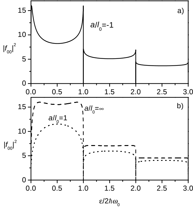
Figure 4.5.2: The function |f_{00}|^2 versus energy. In (a) the parameter a/l_0 = -1 . In (b) the dashed curve corresponds to the unitarity limit ( a/l_0 = \infty ), and the dotted curve to a/l_0 = 1 .
