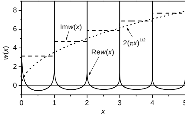
Figure 4.5.1: The functions \text{Re}w(x) (solid curve) and \text{Im}w(x) (dashed lines). The dotted curve shows the function 2\sqrt{\pi x} corresponding to the asymptotic behavior of \text{Im}w at large x .
